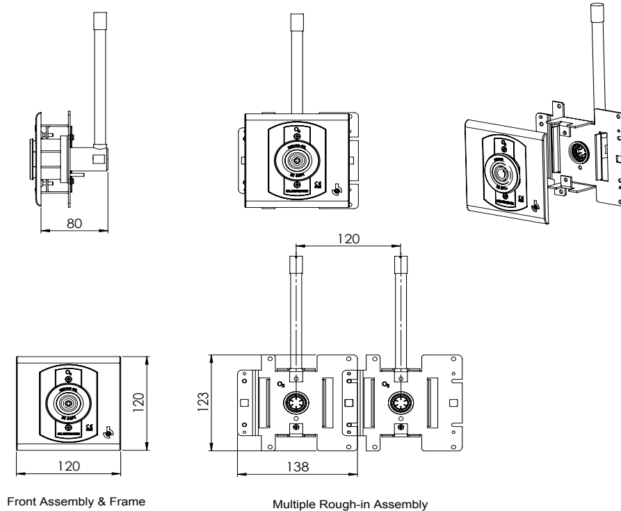
Multiple Rough-in Assembly
